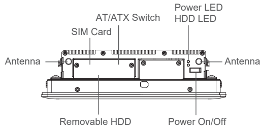
Front I/O
