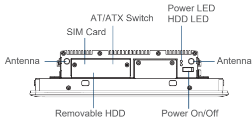
Front I/O
