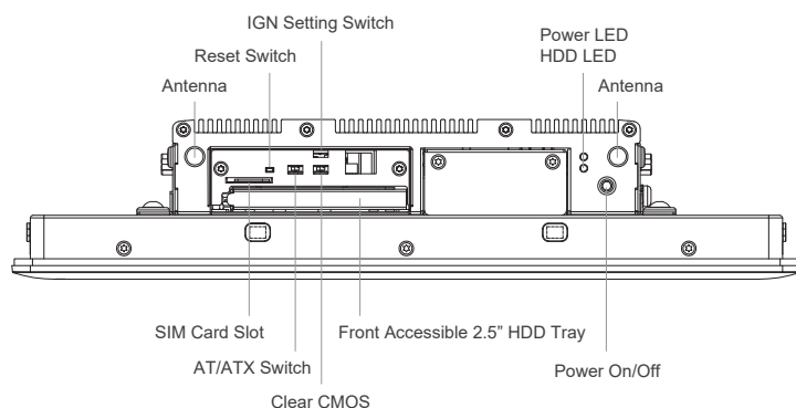
Front I/O
