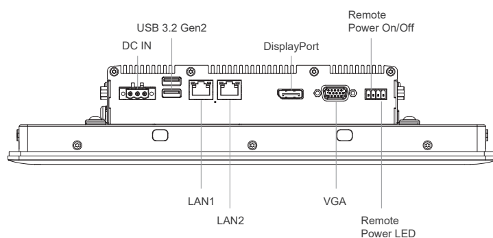
Rear I/O
